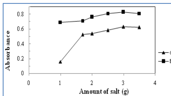
Figure 7. Effect of amount of sodium carbonate on the extraction efficiency; C (Carmoisine), B (Brilliant blue FCF), Experimental conditions: volume of buffer; 7.5 mL, pH of sample; 9, amount of PEG 6000; 3.5 g, temperature; 45°C, 50 ng/mL Carmoisine and Brilliant blue FCF
