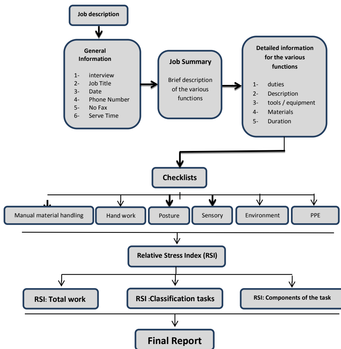
Figure 1. Steps of relative Stress Index (RSI).
