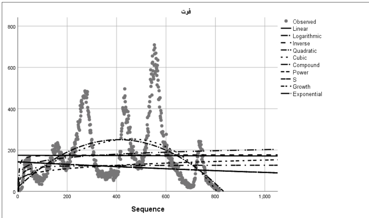
Figure 2. Daily Death Counts and Ten Regression Models Fitted to Data in Iran from the Beginning of COVID-19 to May 15, 2022
