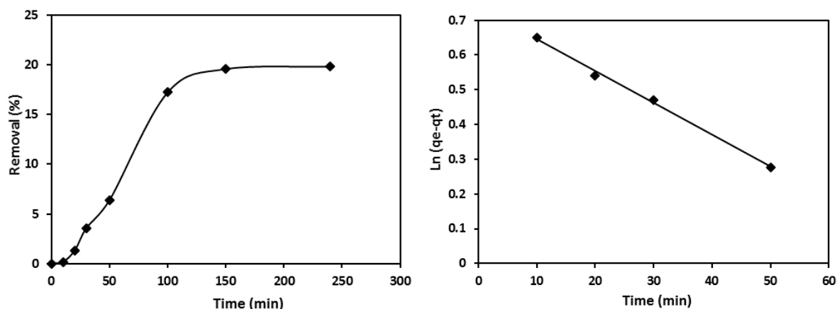
Figure 1. (a) The effects of contact time on lindane adsorption by mineral sand (lindane solution = 100 µg/L, initial pH =7.0, solution volume =250 mL and adsorbent conc. = 2.5 g) and (b) pseudo-first order kinetic model.
